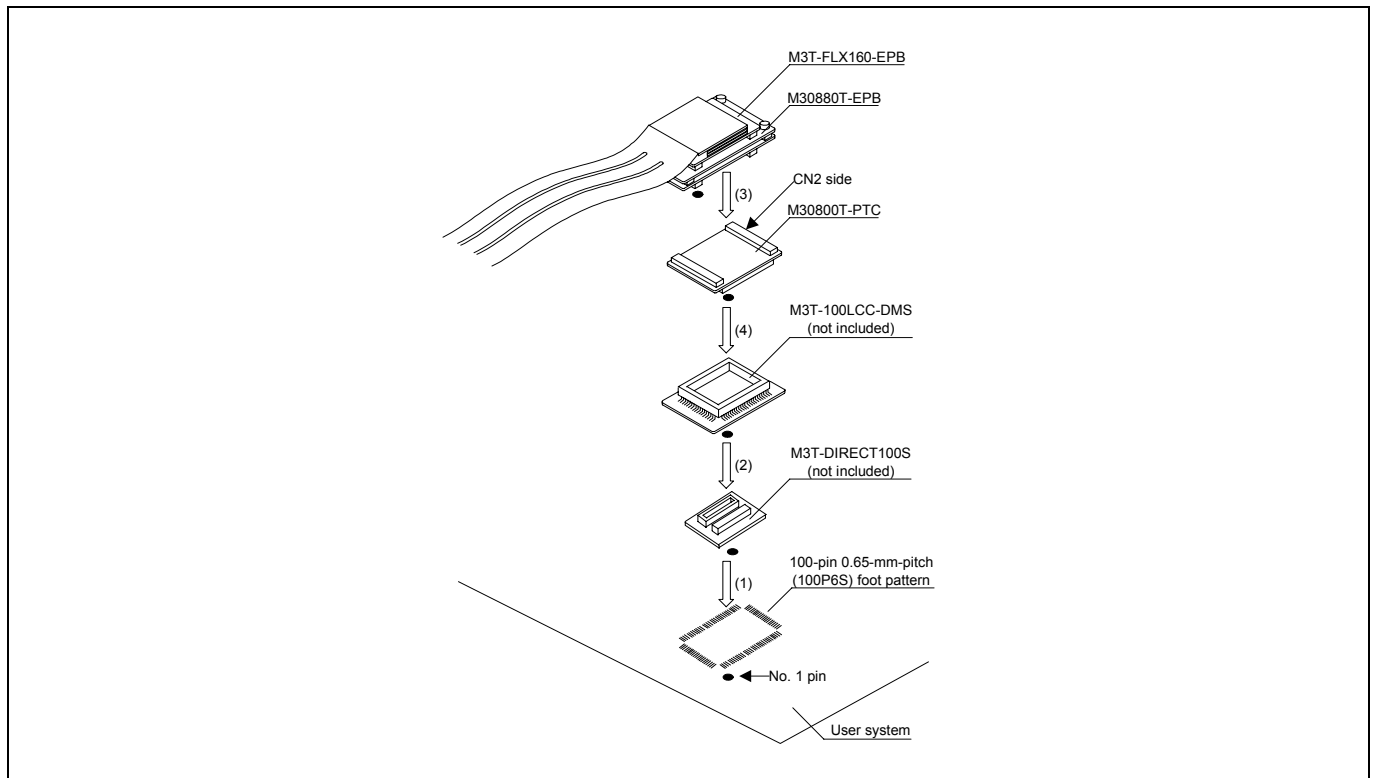
Figure 2.10 Connecting to a 100-pin 0.65-mm-pitch foot pattern (2/3)
